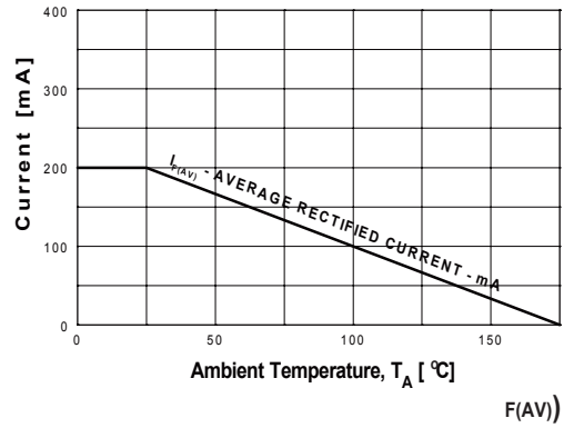
Figure 8. Average Rectified Current (I A ) versus Ambient Temperature (T A )
